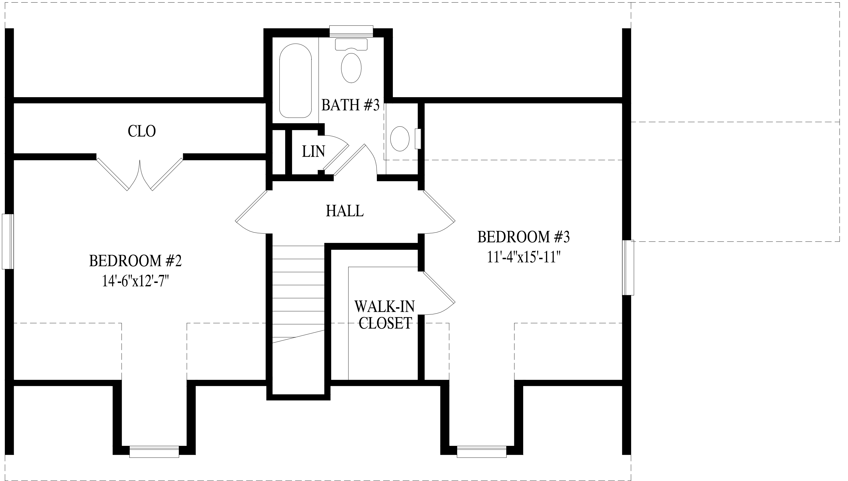
Proposed 2nd Floor - 667 sq. ft.
